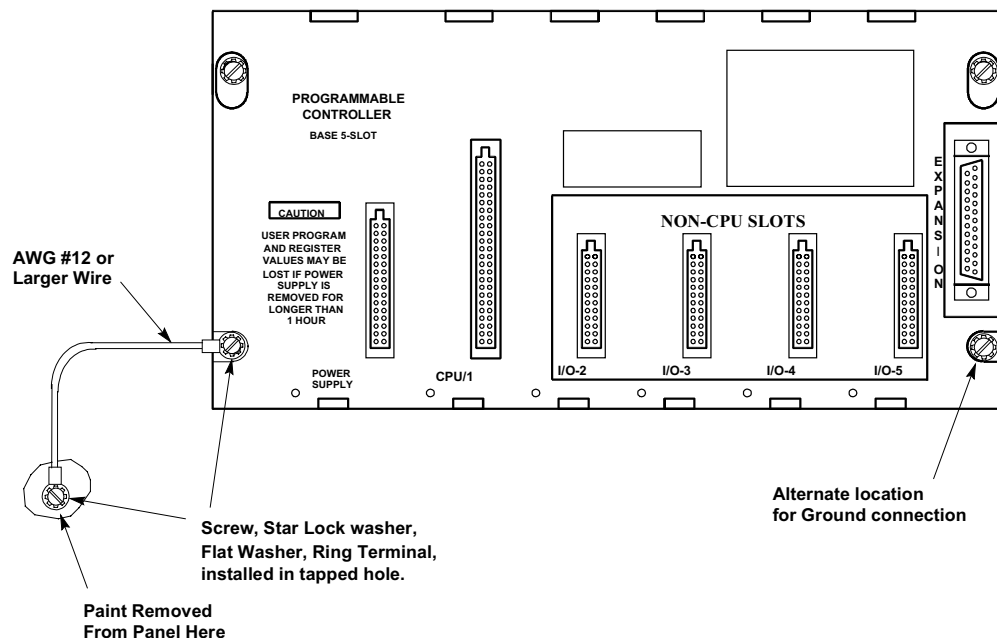
Figure 2-11. Baseplate Grounding
