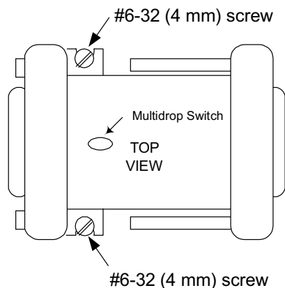
Figure E-4. Mounting Port Isolator to Panel
