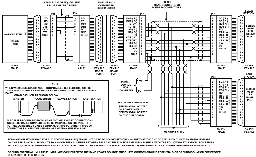
Figure A-7. Workmaster II/Series 90 PLC Multidrop Connection
