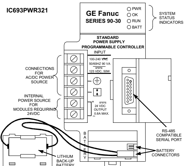
Figure 4-1. Standard AC/DC Input Power Supply - IC693PWR321
