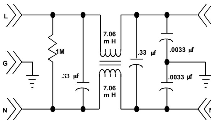
Figure L-2. Equivalent Circuit for 44A720084-001 Line Filter
