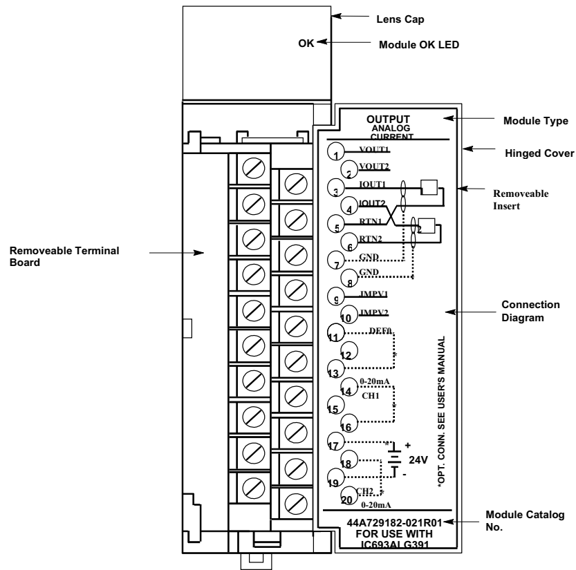
Figure 7-5. Example of Series 90-30 Analog Current Output Module
