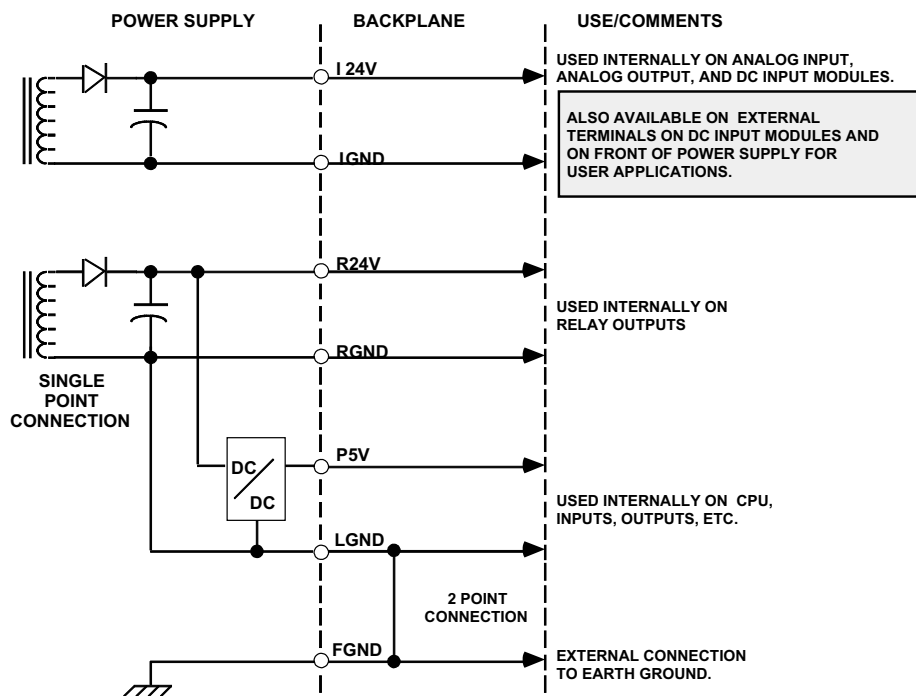
Figure 4-11. Interconnection of Power Supplies
