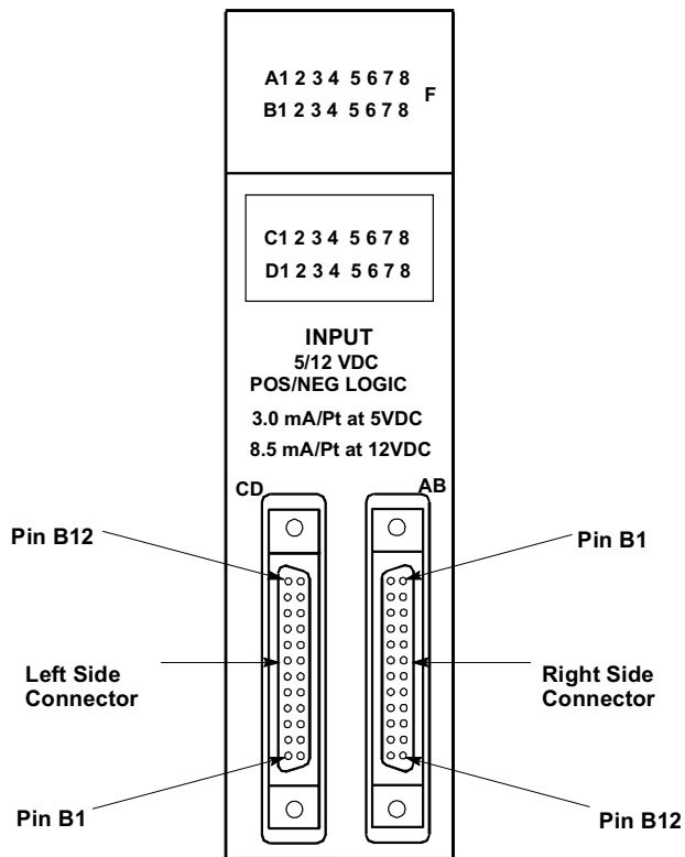
Figure H-8. IC693MDL654 32-Point Module
