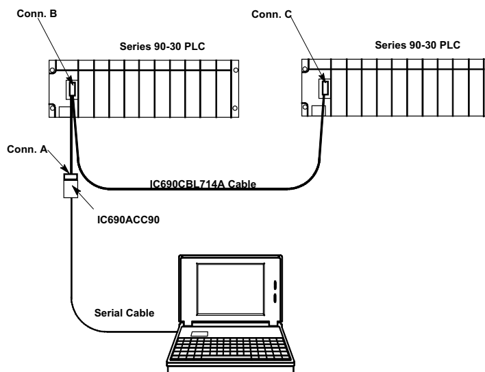
Figure I-5. Multidrop Arrangement for Series 90-30 Redundant System
