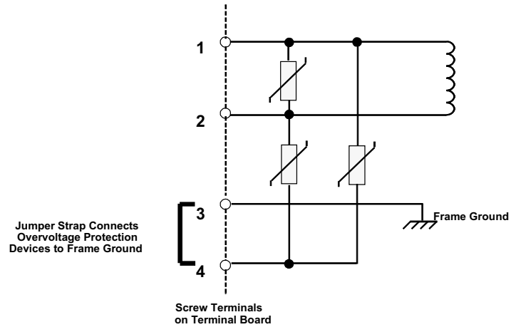
Figure 4-3. Overvoltage Protection Devices and Jumper Strap
