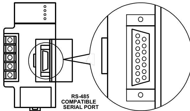
Figure 5-3. CPU Serial Port Connector on Power Supply
