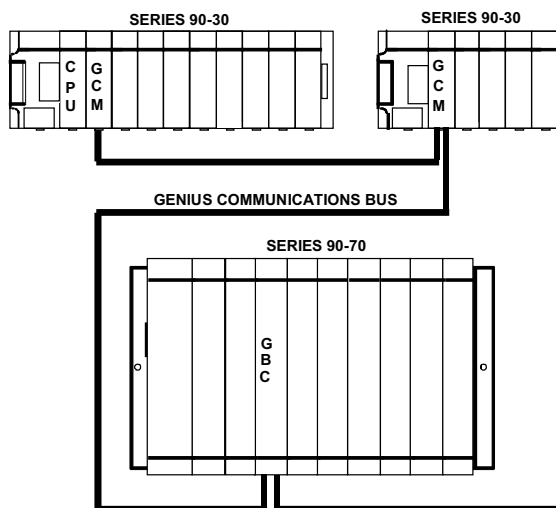
Figure 8-3. Example of Genius Communications Network
