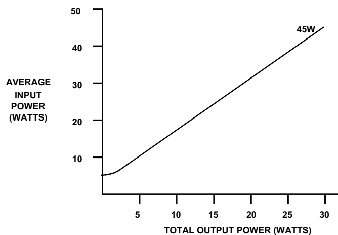
Figure 4-7. Typical Efficiency Curve for IC693PWR328 Power Supply
