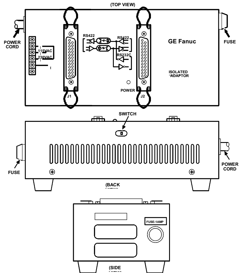
Figure C-1. Isolated/Repeater Converter
