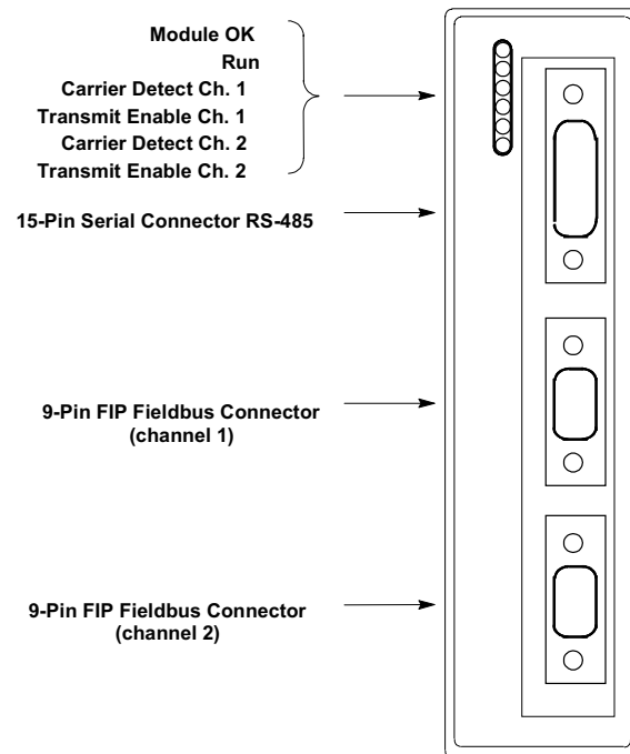
Figure 8-7. Series 90-30 FIP Bus Controller
