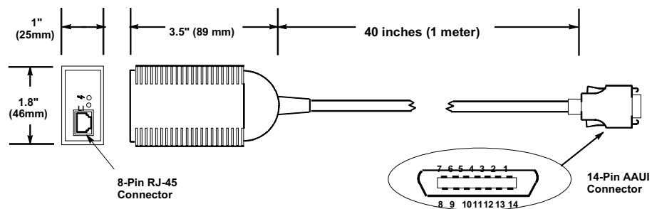
Figure J-1. IC649AEA102 Ethernet 10BASE-T Transceiver
