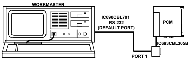
Figure 10-6. PCM to Workmaster Computer or PC-XT Personal Computer
