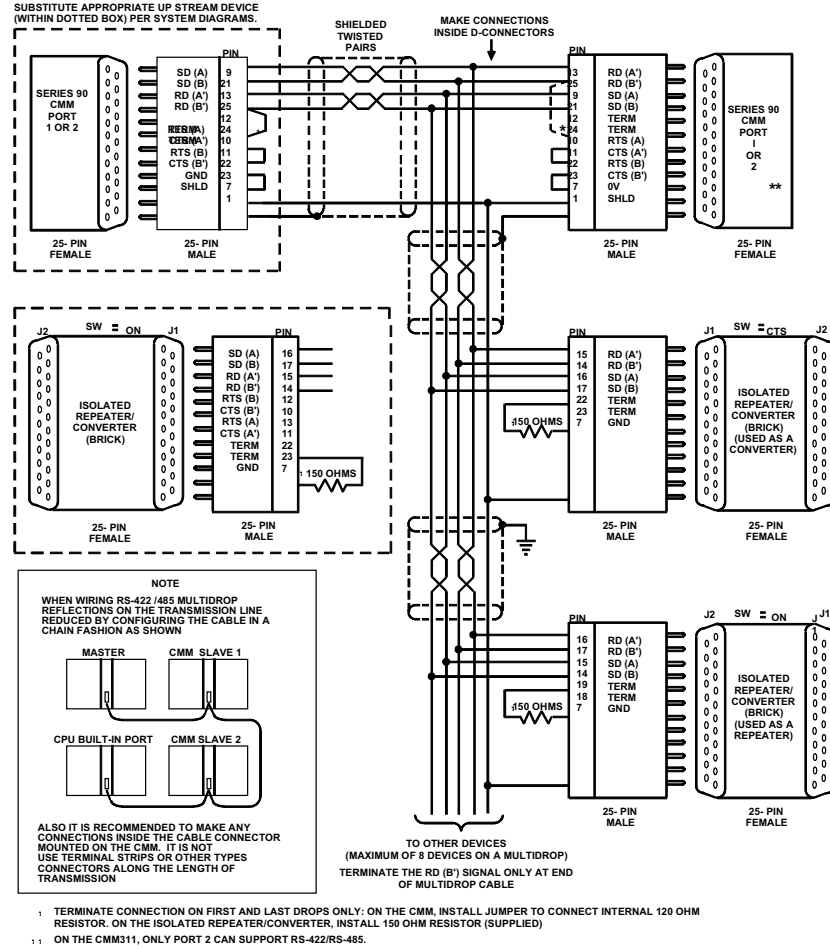
Figure C-8. Cable C; RS422 Twisted Pair
