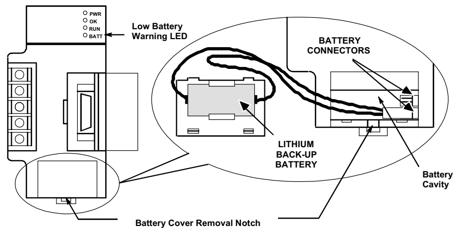
Figure 6-1. Backup Battery for RAM Memory
