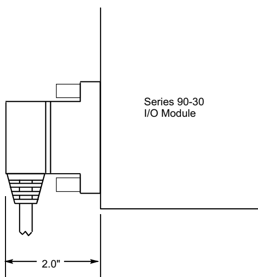
Figure 10-41. Dimension for Depth of Connector
