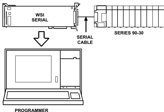
Figure 11-2. Location of WSI in a Series II 90-30 PLC System
