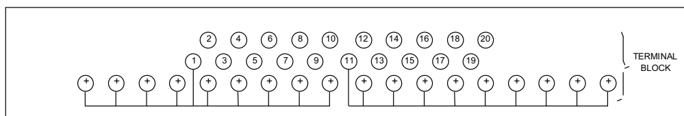
Figure H-5. IC693ACC331 TBQC Terminal Block
