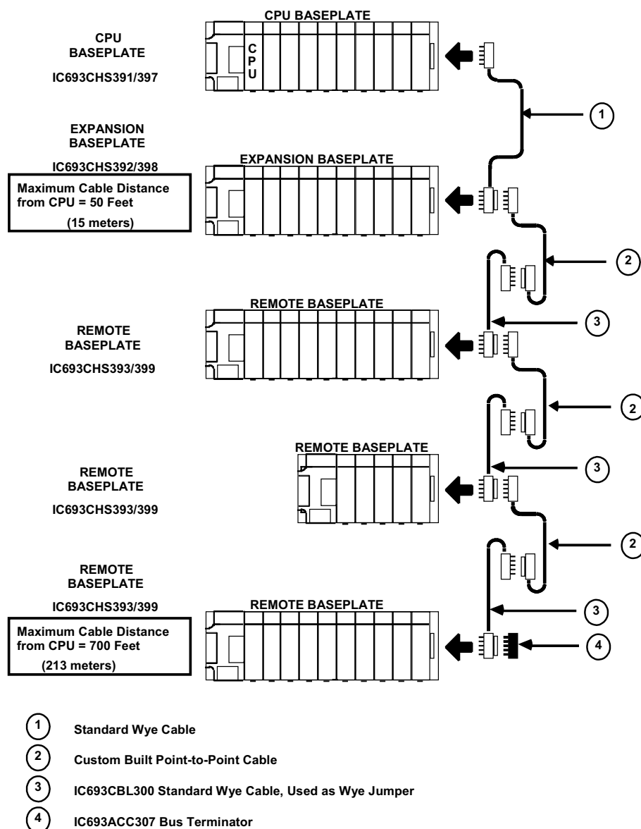
Figure 3-13. Example of Connecting Expansion and Remote Baseplates
