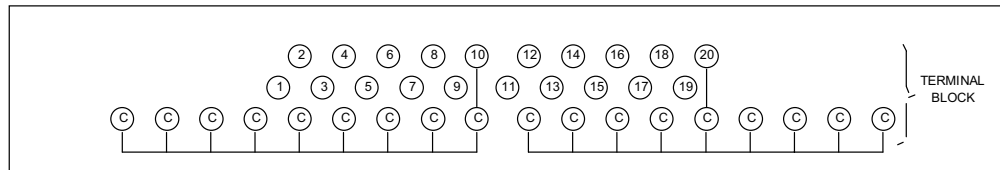
Figure H-4. IC693ACC330 TBQC Terminal Block
