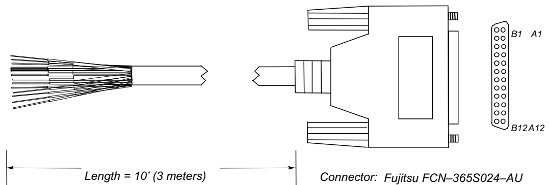
Figure 10-28. IC693CBL310 Cable
