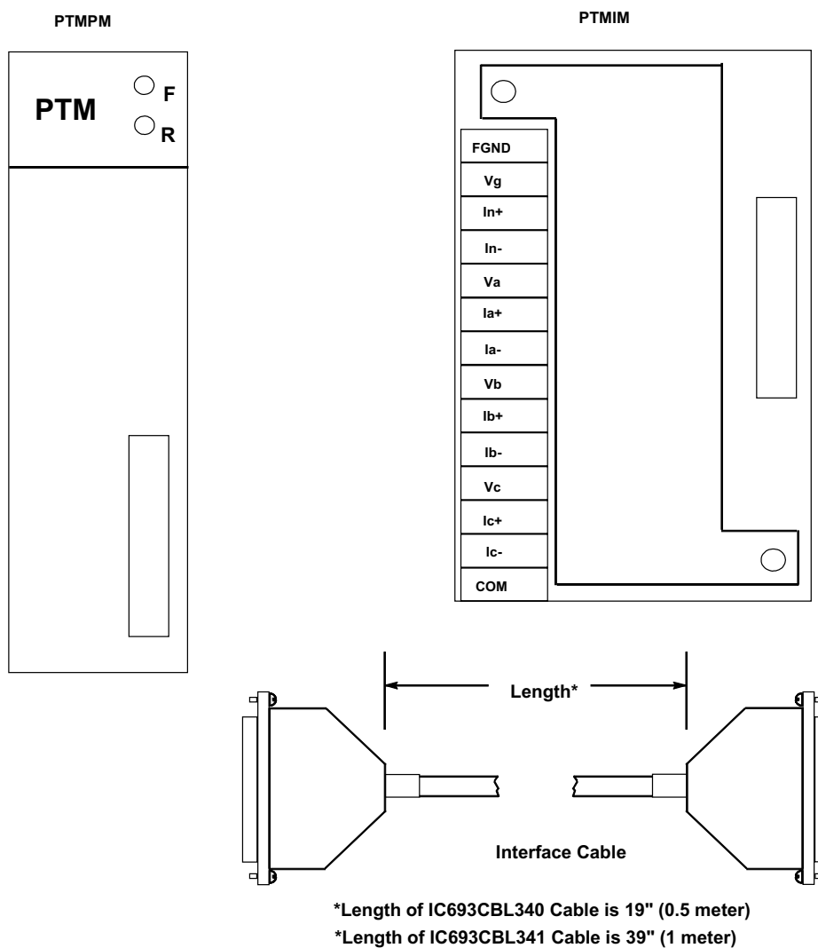
Figure 8-23. IC693PTM100/101 Components
