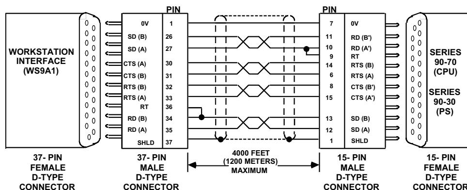
Figure 10-2. Series 90 PLC to Workmaster II Serial Cable
