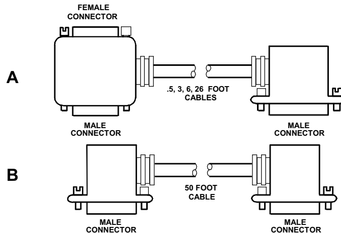
Figure 10-15. Detail of I/O Bus Expansion Cables
