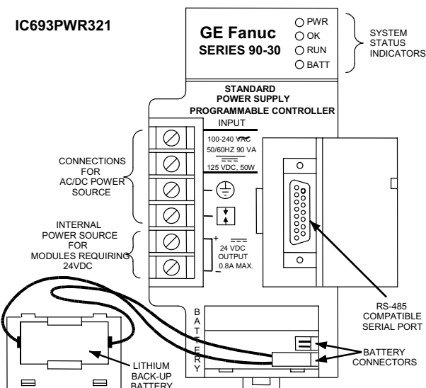
Figure 4-1. Standard AC/DC Input Power Supply - IC693PWR321
