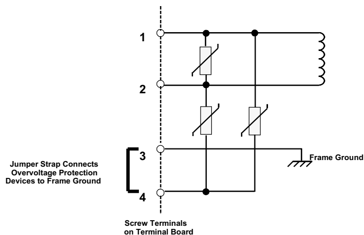
Figure 4-10. Overvoltage Protection Devices and Jumper Strap
