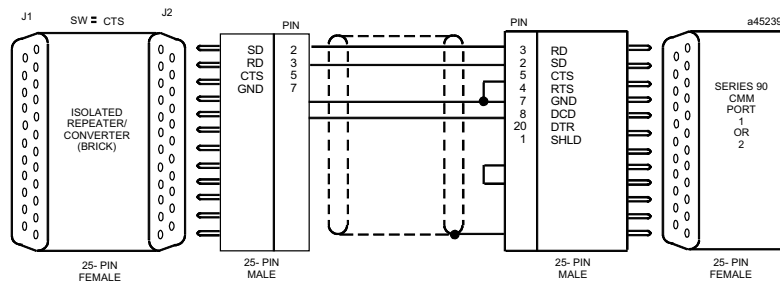
Figure C-10. Cable E; RS-232 Converter to CMM
