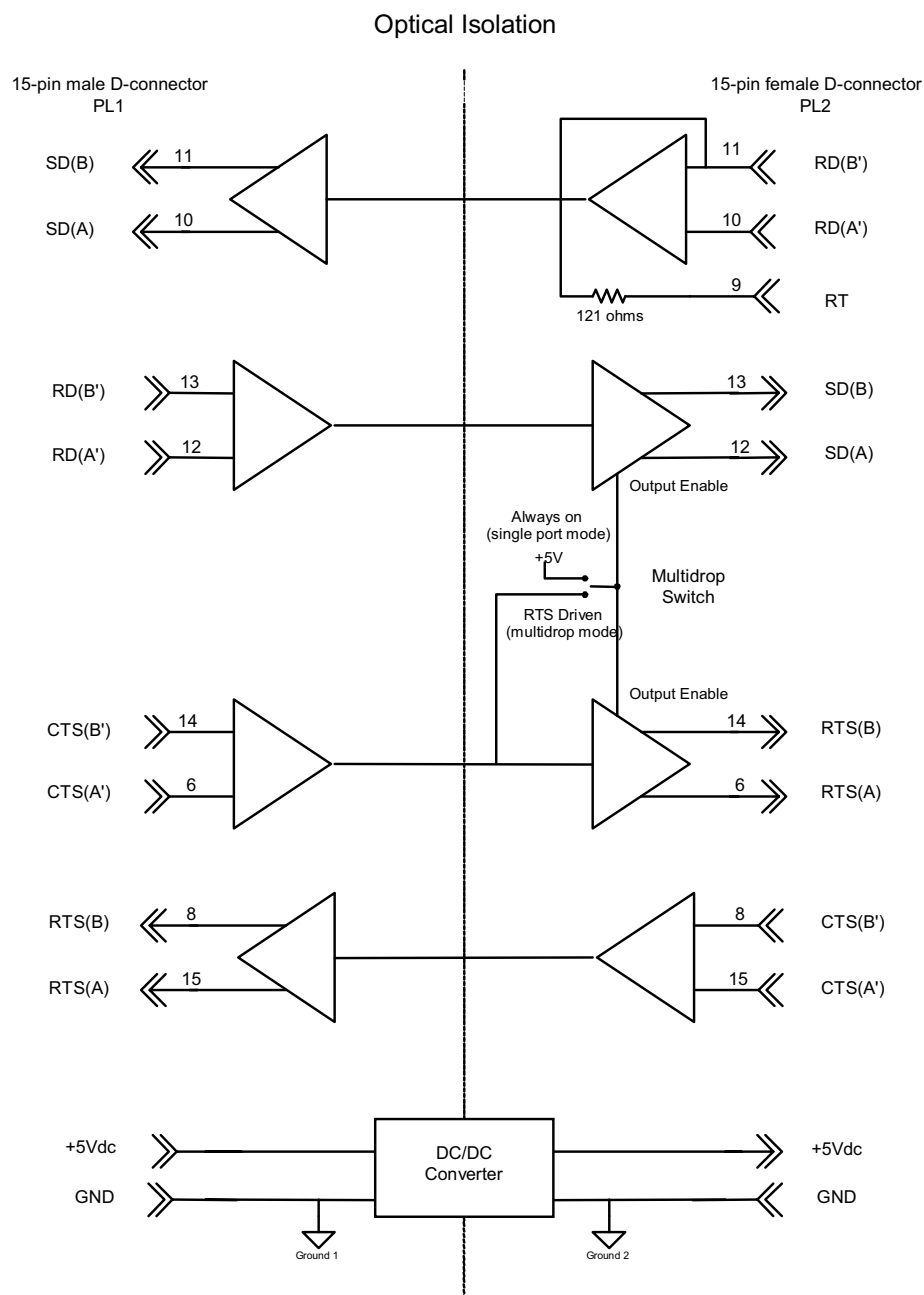
Figure E-2. IC690ACC903 Block Diagram
