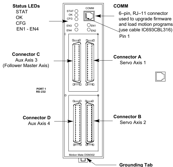
Figure 8-12. Motion Mate DSM302 Module
