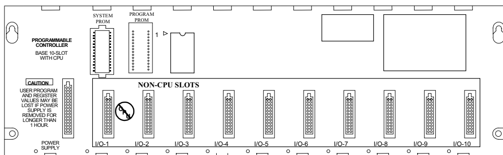
Figure 3-3. Model IC693CPU323 (10-slot) Embedded CPU Baseplate
