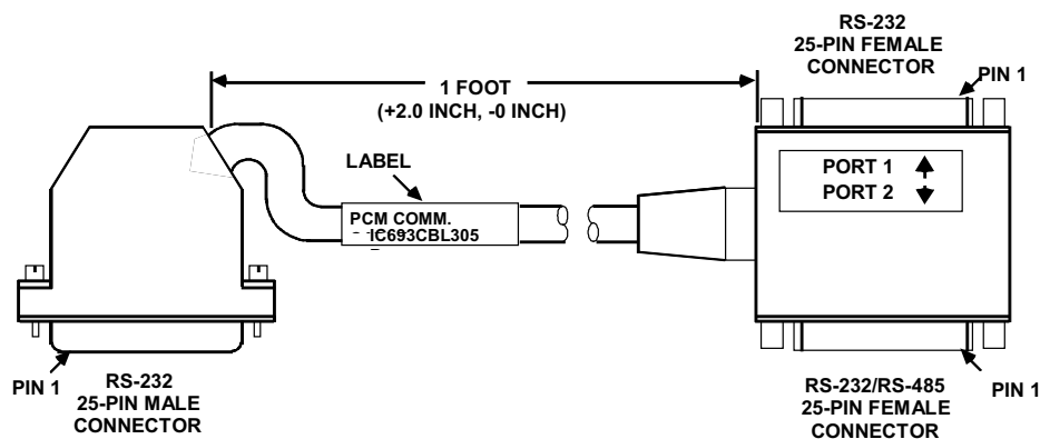
Figure 9-2. IC693CBL305 WYE Cable
