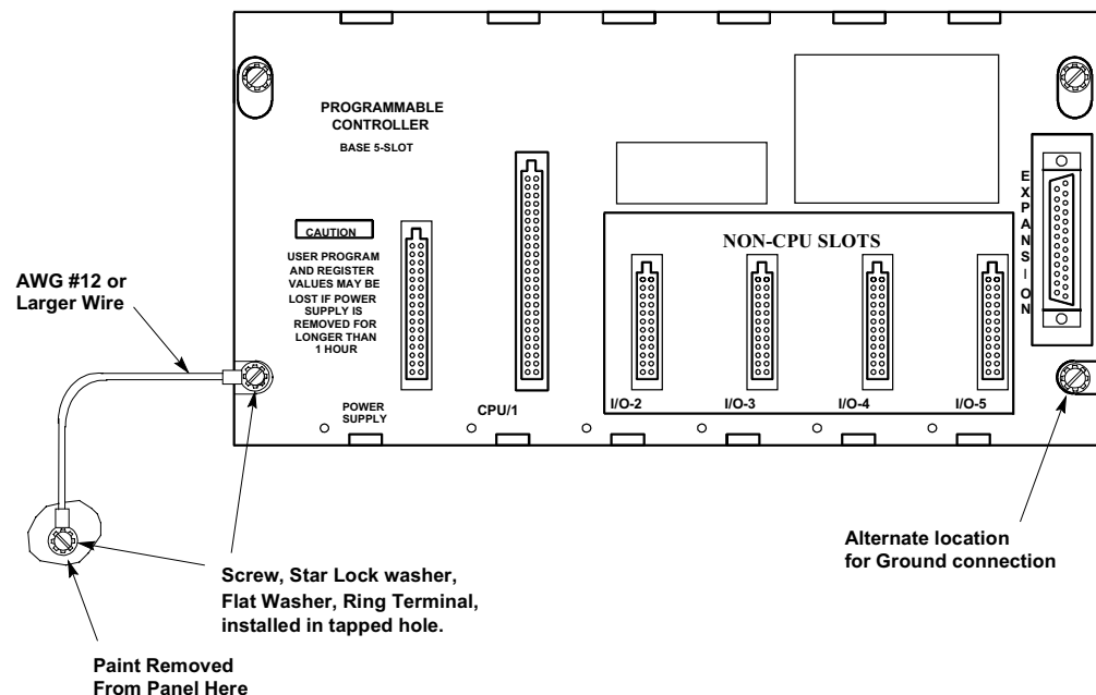
Figure 2-11. Baseplate Grounding
