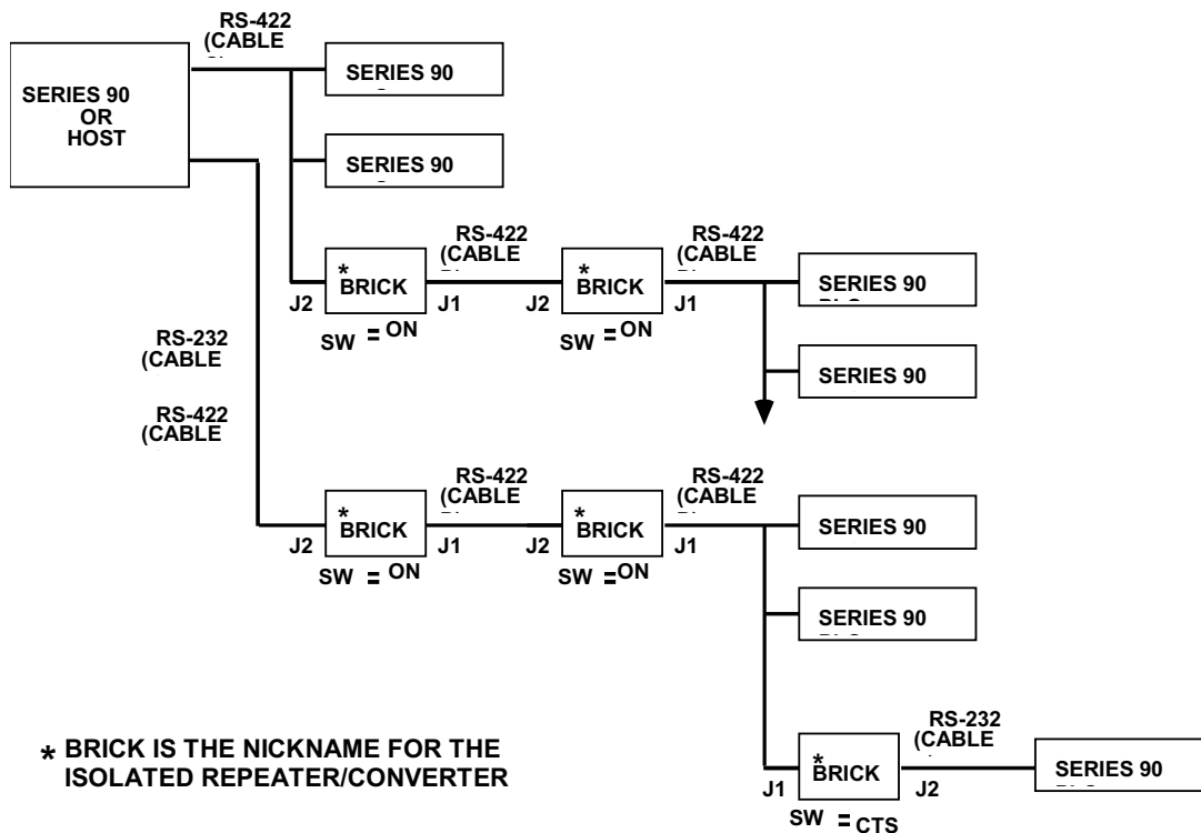
Figure C-5. Complex System Configuration Using the Isolated Repeater/Converter
