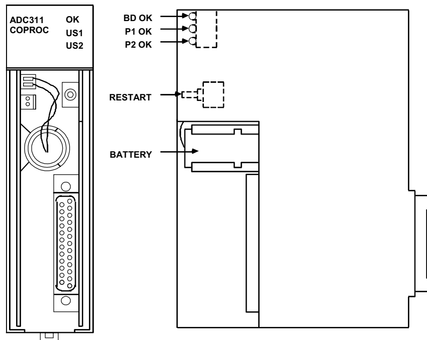
Figure 8-21. Alphanumeric Display Coprocessor Module (ADC)
