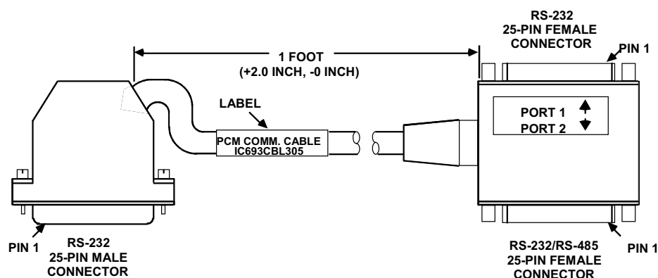
Figure 10-25. Wye Cable
