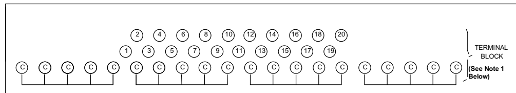
Figure H-6. IC693ACC332 TBQC Terminal Block
