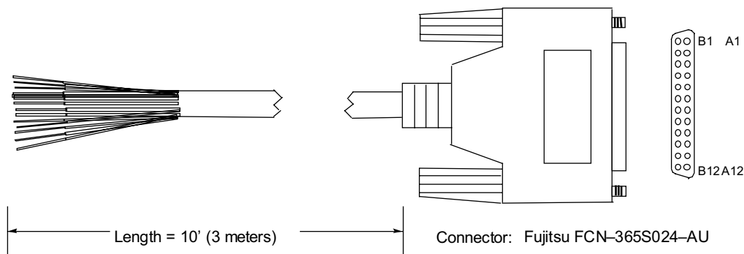
Figure 10-31. IC693CBL315 Cable
