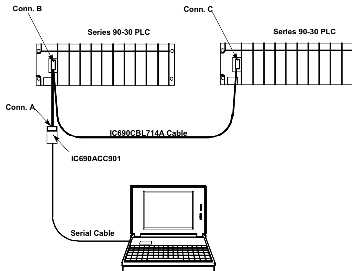
Figure 10-12. Multidrop Arrangement for Series 90-30 Redundant System
