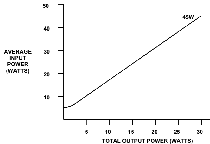
Figure 4-5. Typical Efficiency Curve for 24/48 VDC Power Supply
