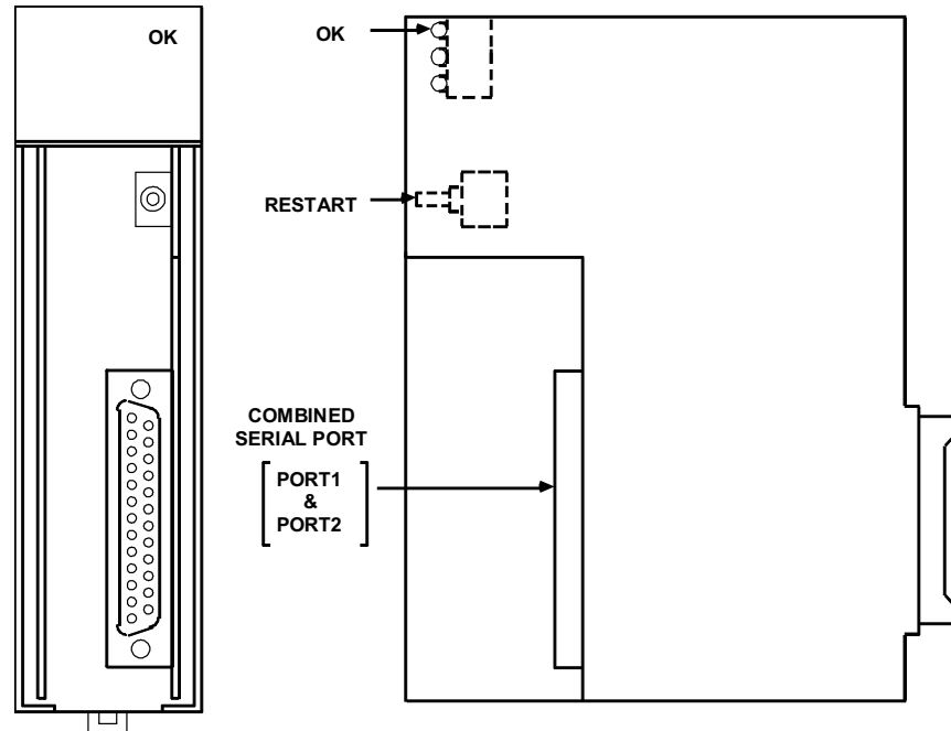
Figure 9-1. AD693CMM301 State Logic Serial Communications Module
