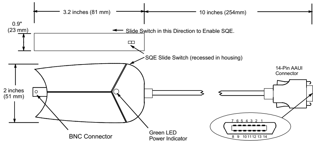
Figure J-2. IC649AEA103 Ethernet 10BASE2 Transceiver
