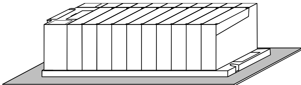
Figure 12-5. Derated PLC Mounting Orientation
