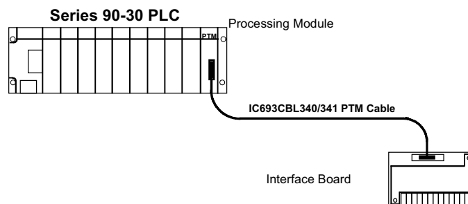
Figure 10-43. PTM Component Mounting and Cable Connection
