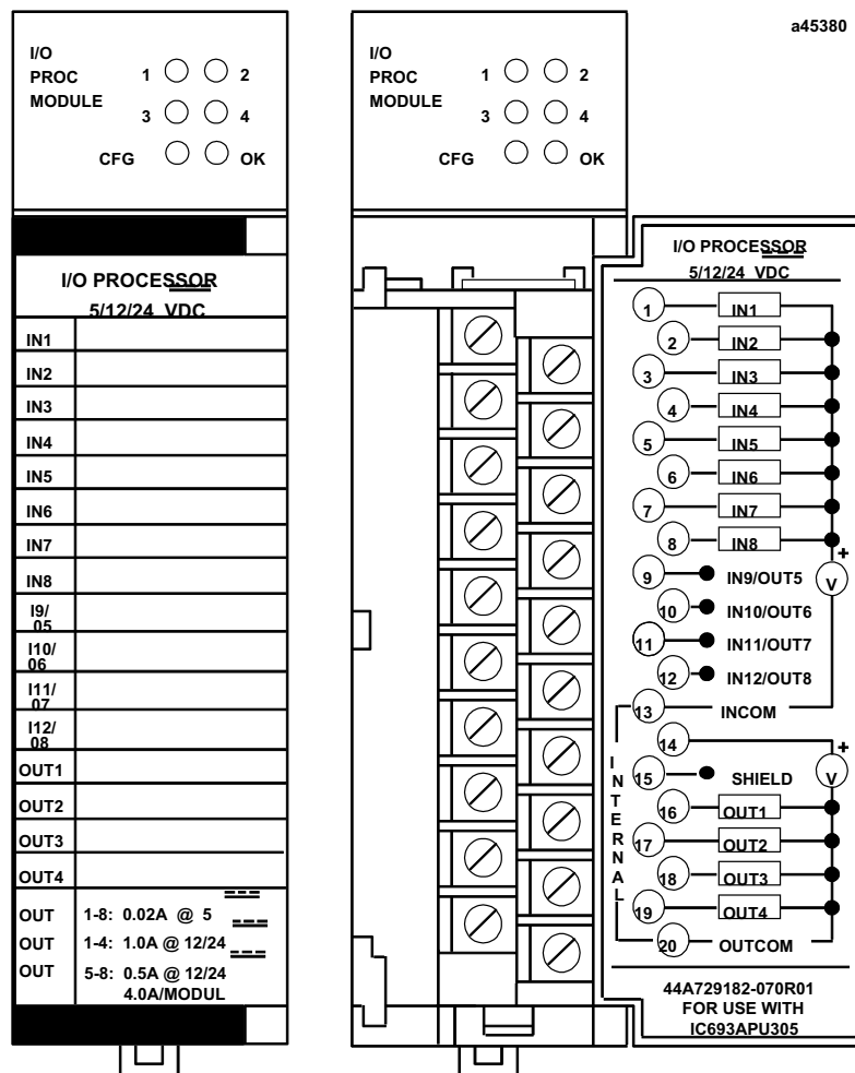
Figure 8-17. I/O Processor Module
