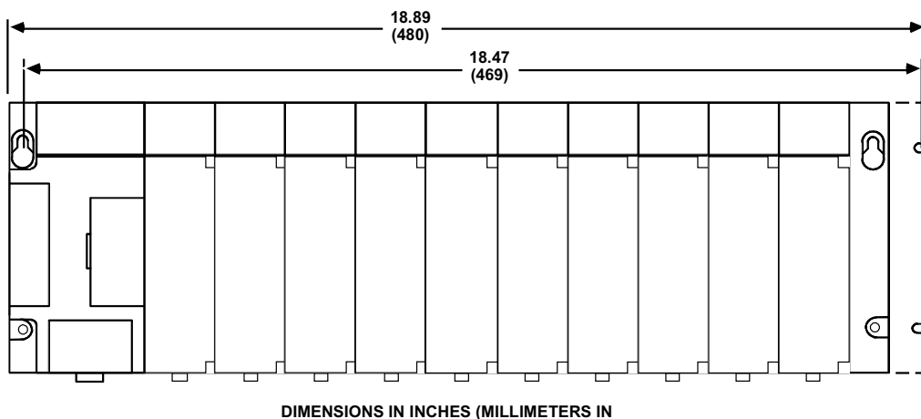
Figure 3-19. Dimensions for 19" Rack Mounting Using IC693ACC308 Adapter Bracket
