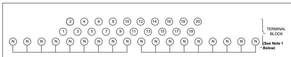
Figure H-7. IC693ACC333 TBQC Terminal Block
