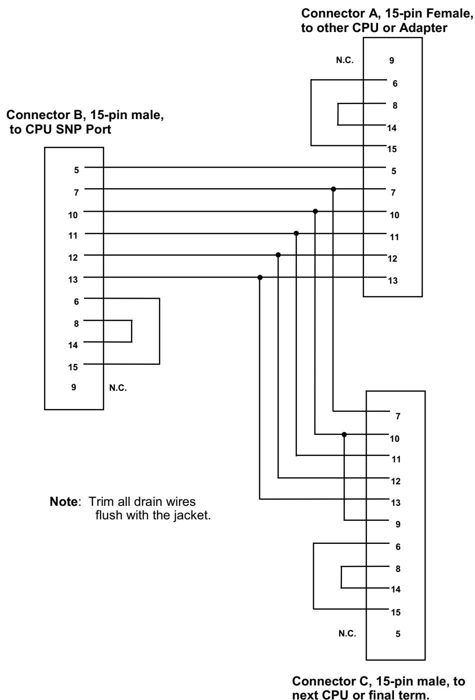
Figure 10-11. Connecting Diagram for Multidrop Cable IC690CBL714A
