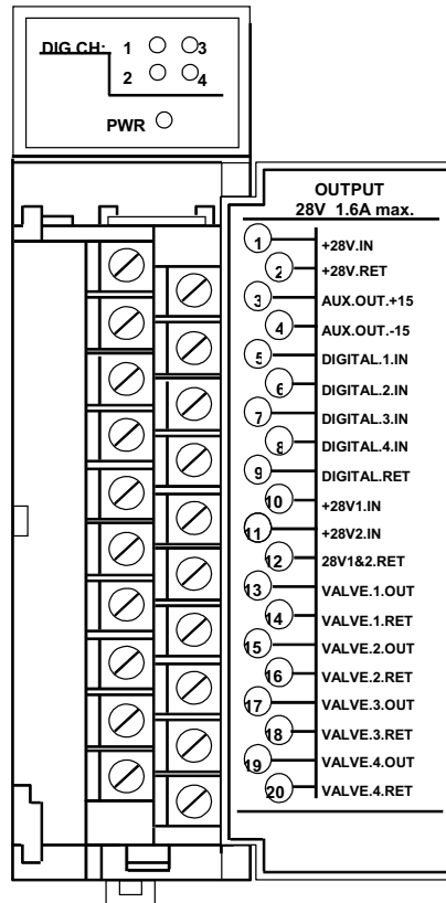
Figure 7-6. IC693DVM300 Digital Valve Driver Module
