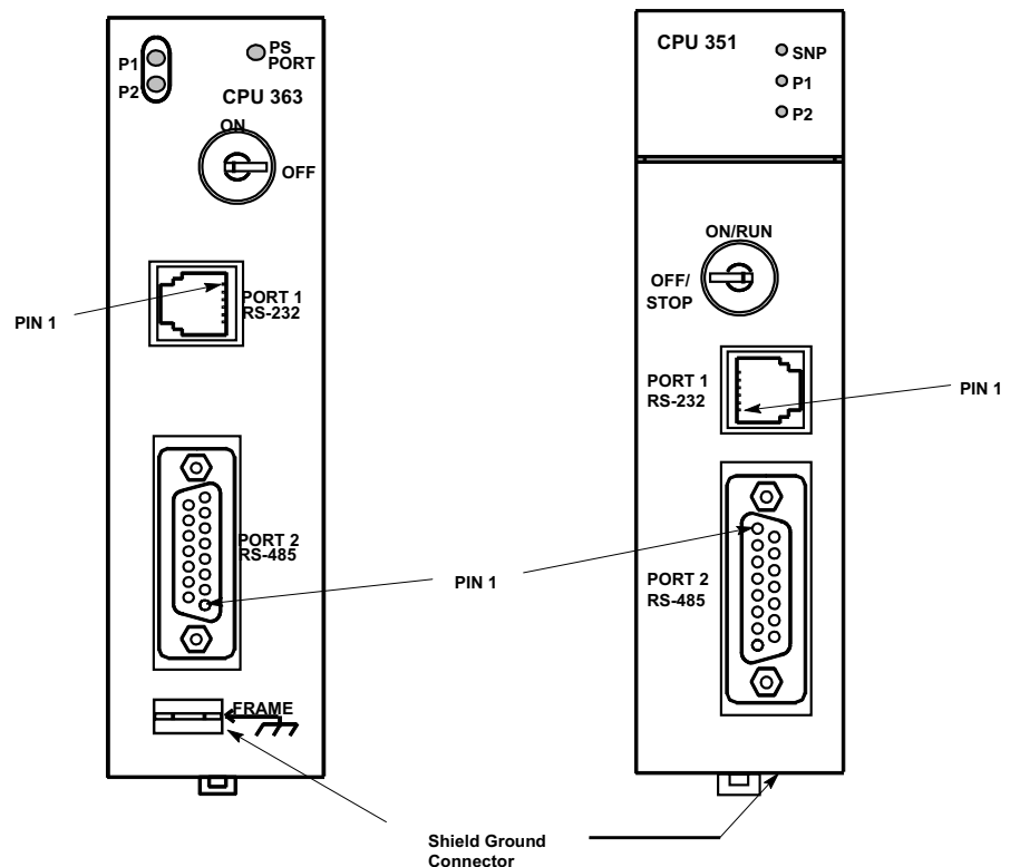
Figure 5-4. CPUs 351, 352, and 363
