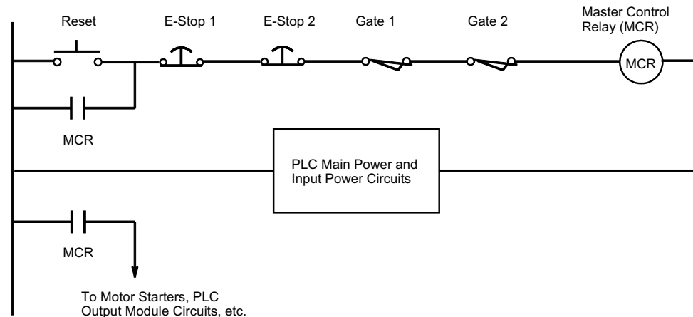
Figure 12-1. Hard-Wired MCR Circuit Example
