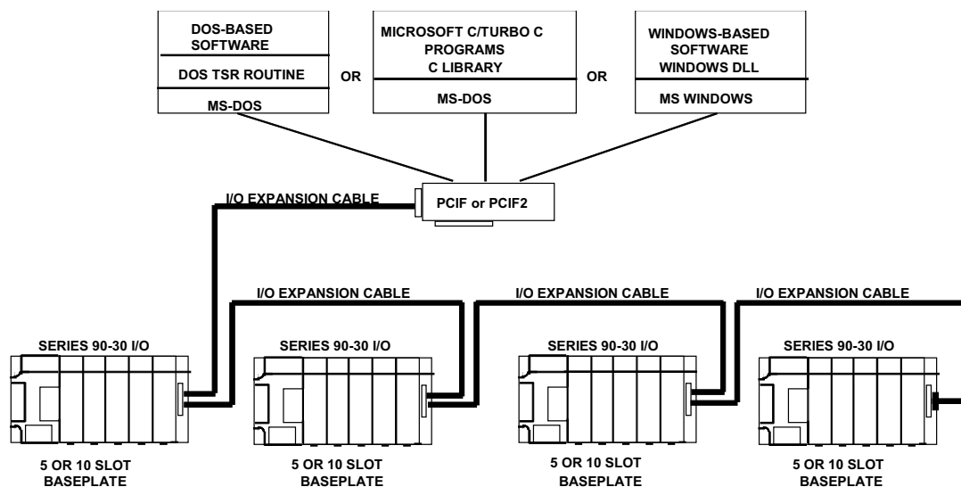
Figure 11-6. Example of PCIF Interface to Series 90-30 I/O
