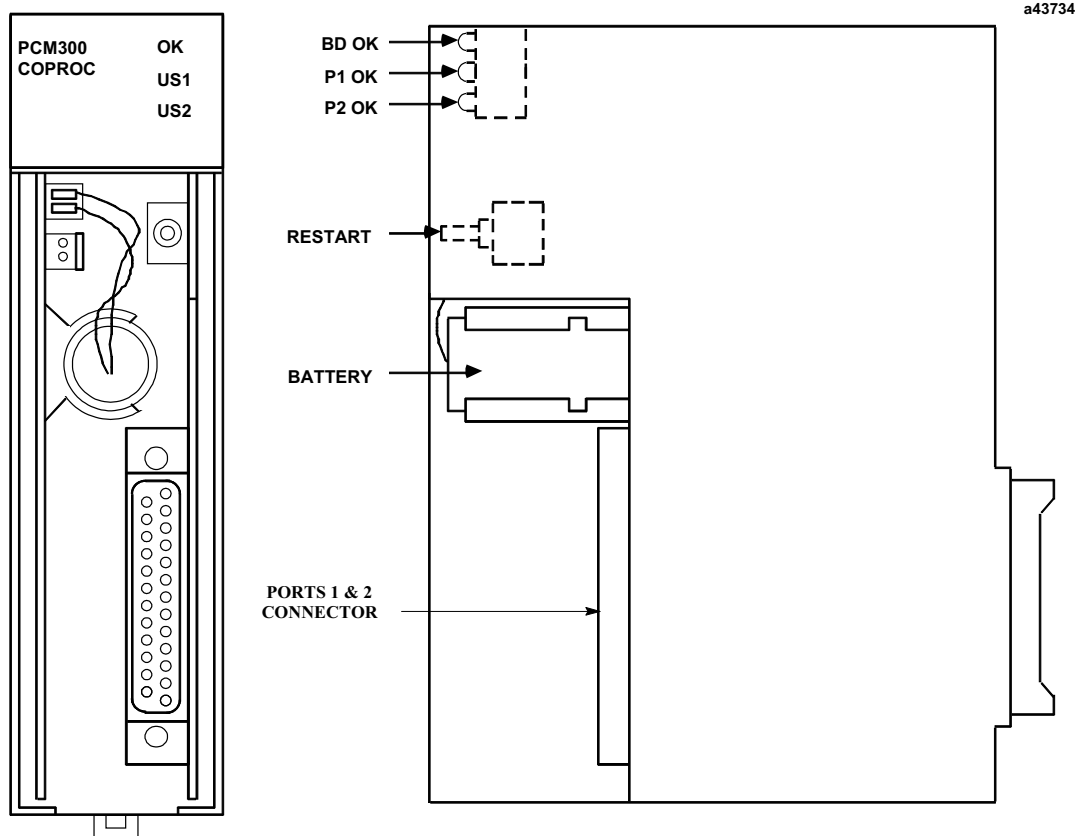
Figure 8-19. Programmable Coprocessor Module (PCM)
