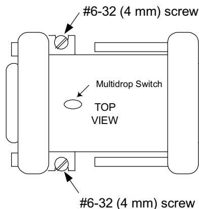
Figure E-4. Mounting Port Isolator to Panel
