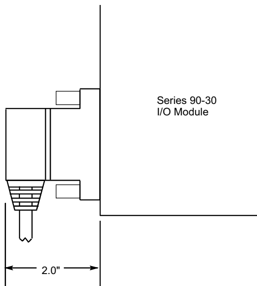
Figure 10-38. Dimension for Depth of Connector for IC693CBL327/328
