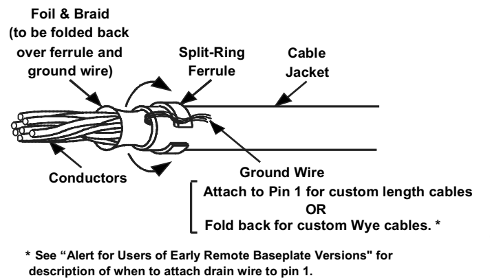
Figure 10-16. How to use Split-Ring Ferrules for Foil and Braided Cable Shield
