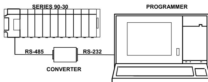
Figure 11-3. Example of IC690ACC900 Converter Connection
