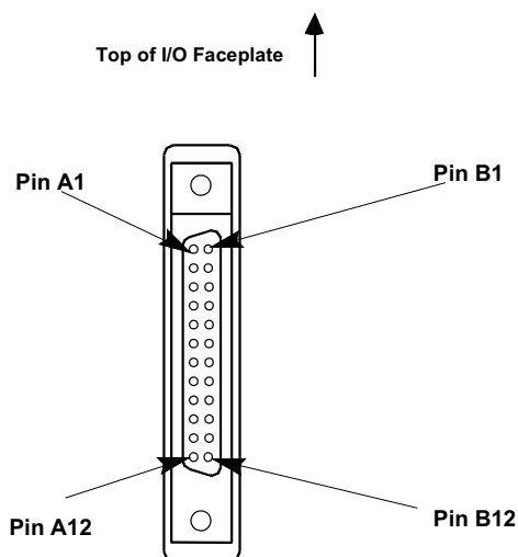
Figure 10-34. Connector Orientation on I/O Faceplate
