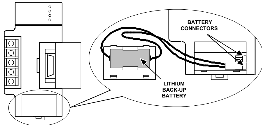
Figure 4-14. Backup Battery for RAM Memory
