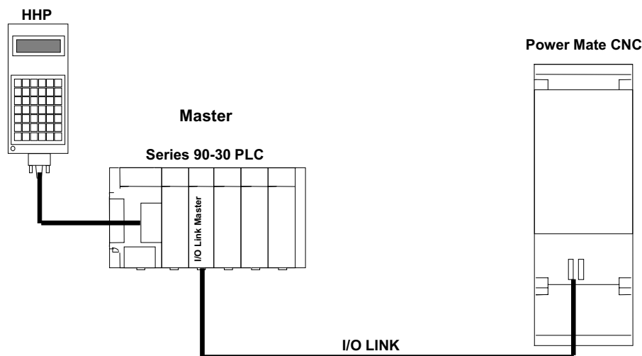
Figure 8-16. Example of I/O LINK Master System Configuration
