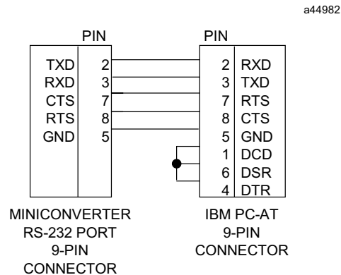
Figure D-2. Miniconverter to PC-AT
