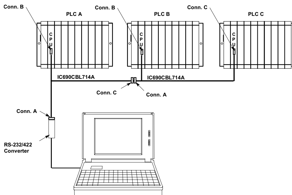
Figure 10-14. Multidrop Arrangement for Series 90-70 TMR Redundant System
