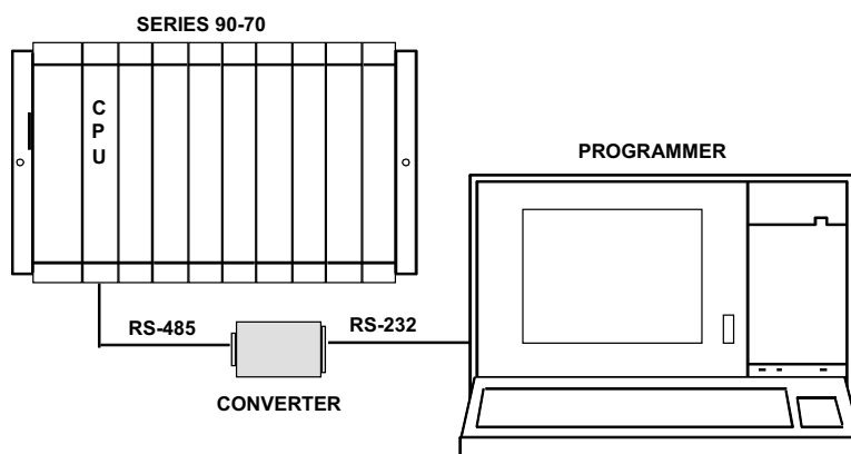
Figure B-2. Typical Configuration with Series 90-70 PLC
