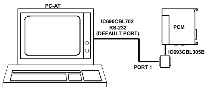
Figure 10-8. PCM to PC-AT Personal Computer
