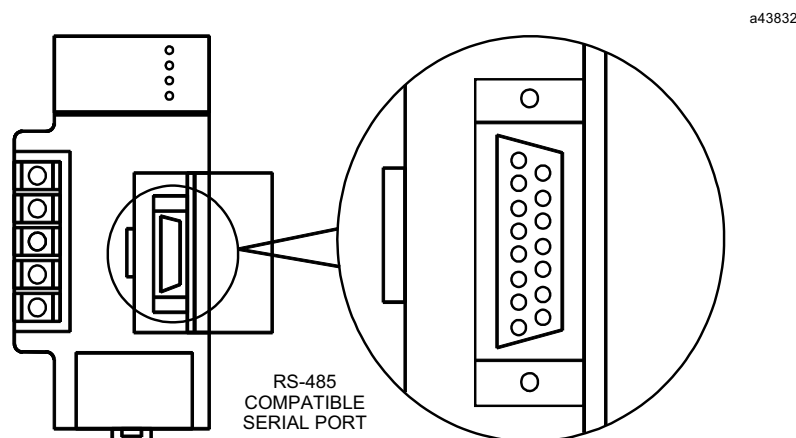
Figure 4-13. Serial Port Connector
