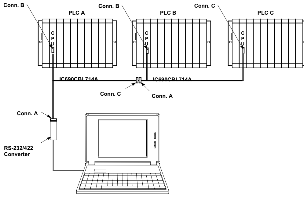
Figure I-4. Multidrop Arrangement for Series 90-70 TMR Redundant System
