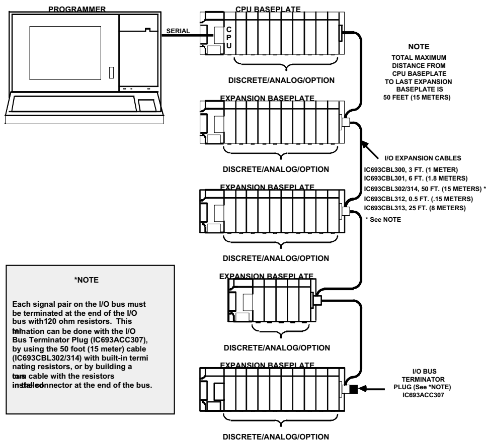
Figure 10-21. Example of Connecting Expansion Baseplates
