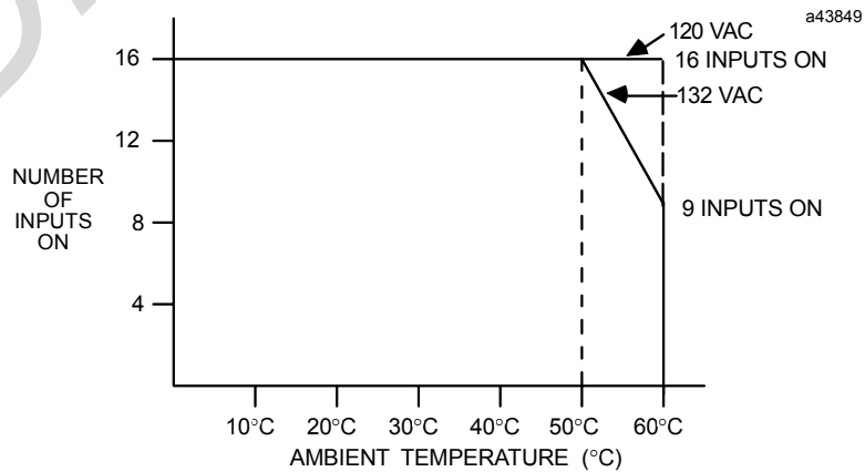
Figure 6-4. Input Points vs. Temperature for IC693MDL240
