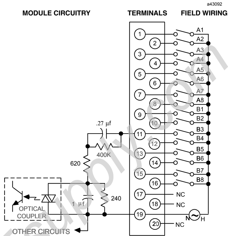
Figure 6-3. Field Wiring - 120 Volt AC Input Module - IC693MDL240
