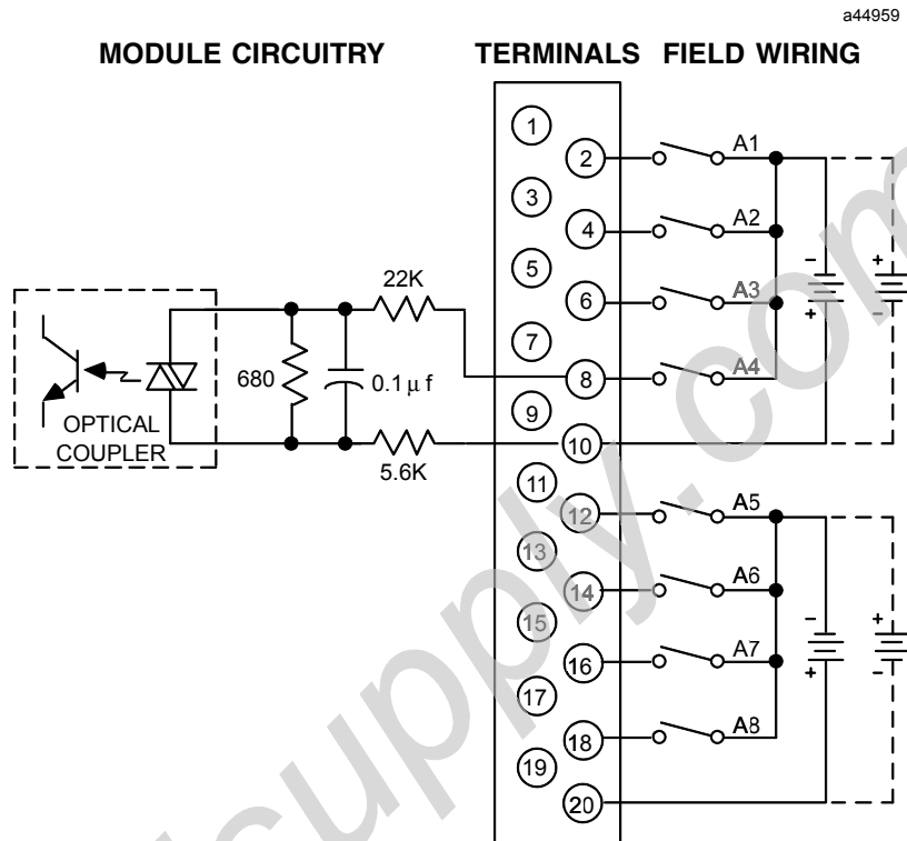
Figure 6-7. Field Wiring - 125 Volt DC Positive /Negative Logic Input Module - IC693MDL632
