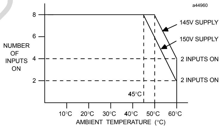
Figure 6-8. Input Points vs. Temperature for IC693MDL632
