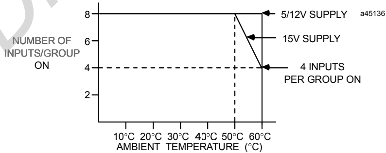
Figure 6-17. Input Points vs. Temperature for IC693MDL654
