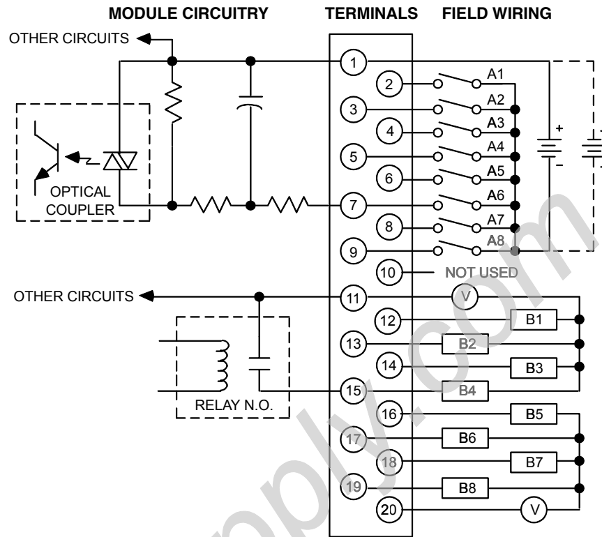
Figure 8-2. Field Wiring 24 VDC Input/Relay Output Module - IC693MDR390
